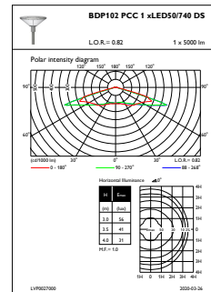
OFPL1_BDP102PCC1xLED50740DS
