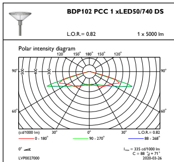
OFPC1_BDP102PCC1xLED50740DS
