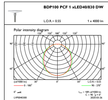
OFPC1_BDP100PCF1xLED40830DW
