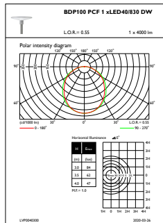
OFPL1_BDP100PCF1xLED40830DW
