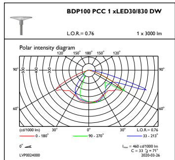
OFPC1_BDP100PCC1xLED30830DW
