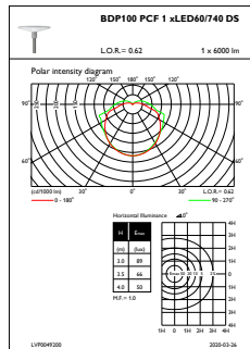
OFPL1_BDP100PCF1xLED60740DS
