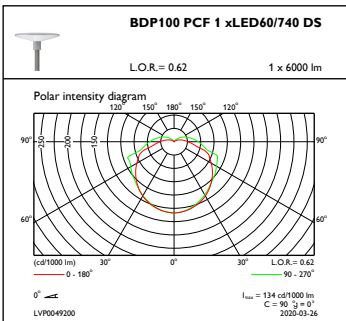
OFPC1_BDP100PCF1xLED60740DS
