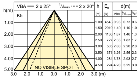
LDDBE_CDMR111E_0003-Beam diagram
