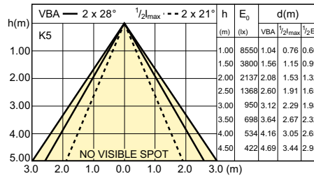
LDDBE_CDMR111E_0009-Beam diagram
