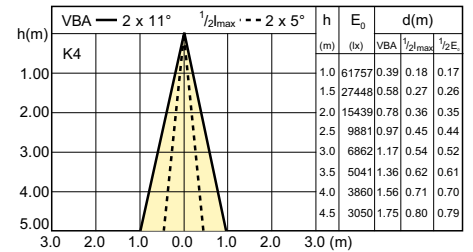
LDDBE_CDMR111E_0007-Beam diagram
