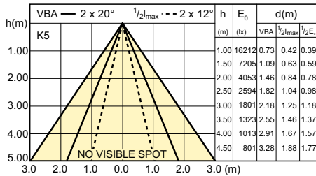
LDDBE_CDMR111E_0008-Beam diagram
