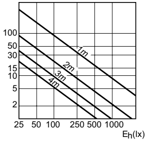
LDAC_CDMR111E_0002-Accent diagram
