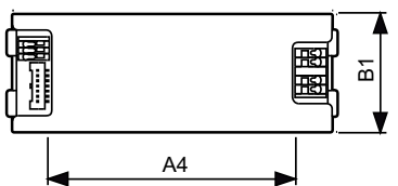
LCN8600/00 MultiOne interface USB2DALI
