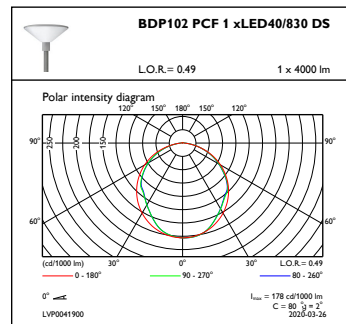
OFPC1_BDP102PCF1xLED40830DS
